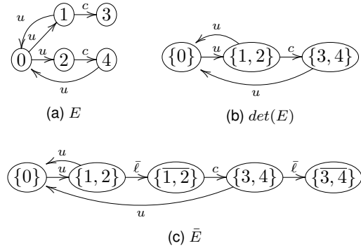
Fig. 3: Determinisation Example
