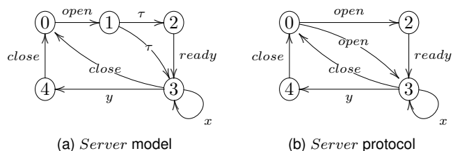
Fig. 1: Motivating Example
